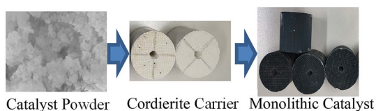
Fig. 3 Preparation process of the monolithic catalyst
